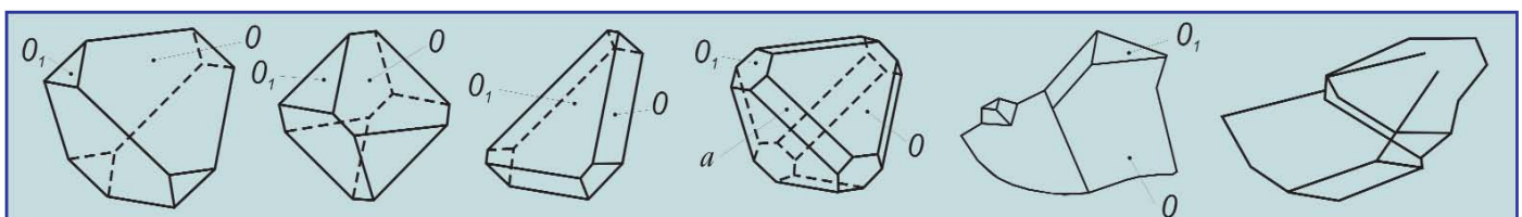
CBN - Kristallformen.
